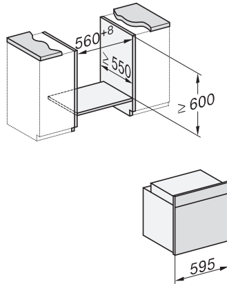
H226x-1B/BP/E/EP/MP, H2x6xB/BP, H7x6xB/BP/BPX, installation drawings
