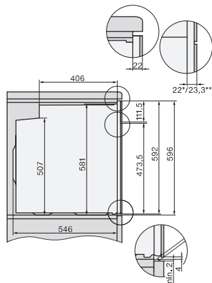
side view H7000 XL built-under, installation drawing
