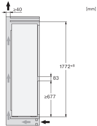
KD7713E Active, KDN7713E Active, side view (installation drawings)
