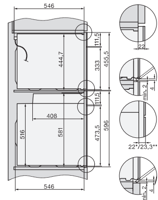
H2xxx-1 B/BP/E/MP, H7xxx B/BP/BM/BMX, installation drawings
